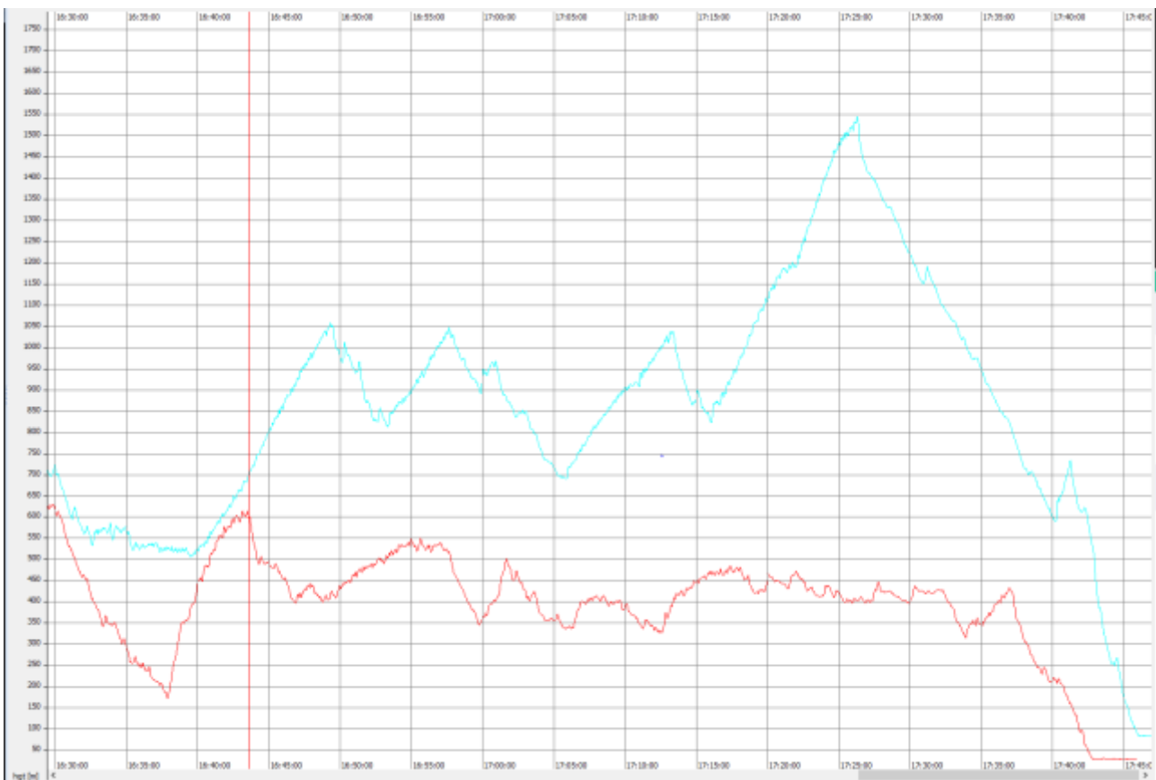
Figure 9: Barogram of GT and VS on task 3 after passing turning point "208Paseimeniai"
